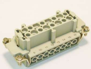
RPM0066 B16 Female Insert 16 amp TC8CxxG Thermocouple Cables (DME primary supplier: Harting)
