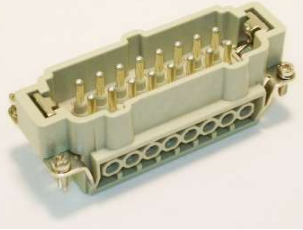
RPM0063 B16 Male Insert 16 amp MTC8G Mold Thermocouple Connector (DME primary supplier: Harting)
