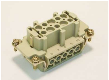
RPM0065 B10 Female Insert 16 amp TC5CxxG Thermocouple Cables (DME primary supplier: Harting)
