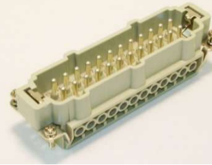
RPM0064 B24 Male Insert 16 amp MTC12G Mold Thermocouple Connector (DME primary supplier: Harting)
