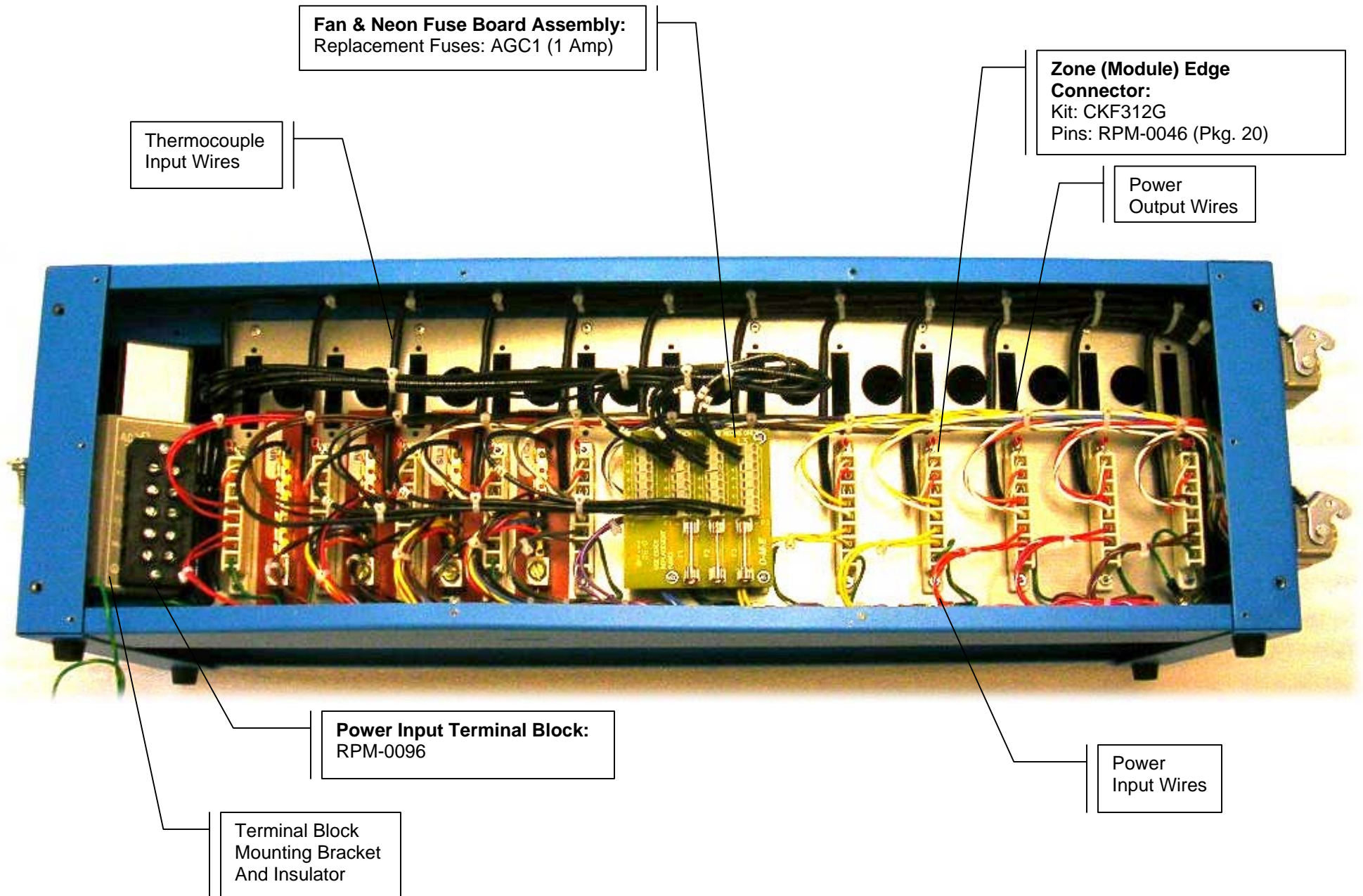
MFP12G MAINFRAME – REAR VIEW
